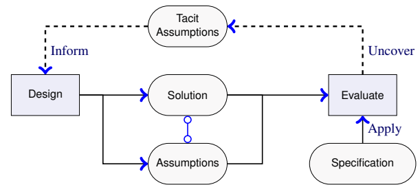
Fig. 4. Solutions implement specifications. The assumptions delineate the limitations of the solution artifact, and should be more general for a solution than for the specification.
