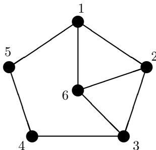
Figure 2: Replicating one vertex in a 5-hole.
