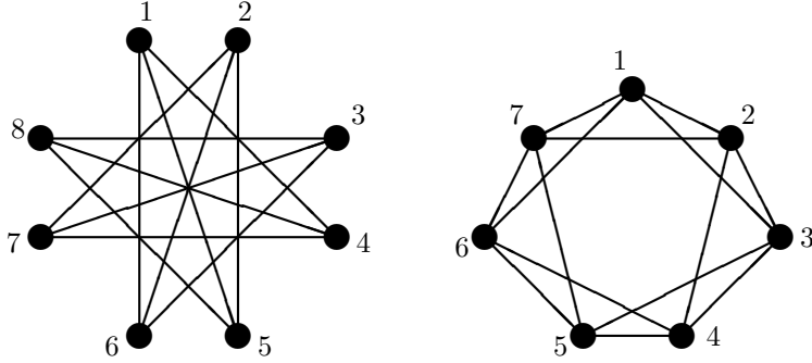
Figure 1: An (8, 3) -web and a (7, 3) -antiweb.
