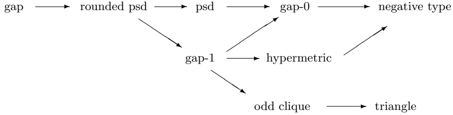
Figure 1: Inequalities for the cut polytope.
