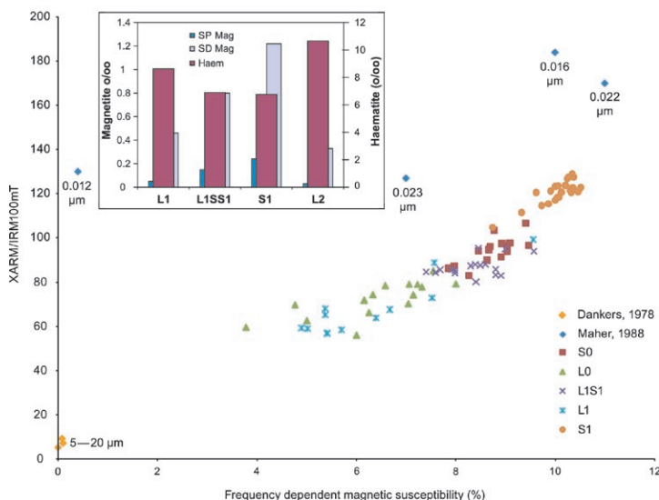
FIGURE 3 \chi_{ARM}/IRM_{100mT} versus frequency-dependent susceptibility for samples of loess and palaeosol, central Loess Plateau, and, for comparison, magnetite powders of known grain size. Compared with the \chi_{ARM}/IRM values for the pure, grain-sized magnetite, the loess and palaeosols show some offset, because they also contain some hematite/goethite. Inset: mathematical unmixing of the magnetic minerals and grain sizes in loess unit 1 ( L_1 ), an incipient soil within L_1 ( L_1SS_1 ), the last interglacial palaeosol ( S_1 ), and loess unit 2 ( L_2 ) (Maher and Thompson 1992)
