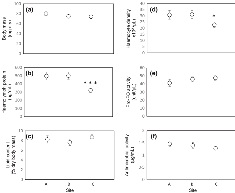
Figure 1 Body condition and immune traits at the three populations. (a) Mean body mass ( \pm SE), (b) mean haemolymph protein content ( \pm SE), (c) mean body lipid content ( \pm SE), (d) mean total haemocyte density ( \pm SE), (e) mean prophenoloxidase activity ( \pm SE) and (f) mean lysozyme-like antimicrobial activity ( \pm SE). Asterisks indicate significant differences.
