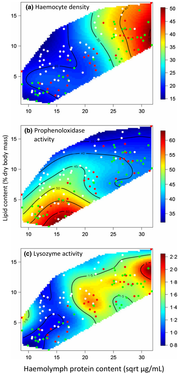
Figure 4 Thin-plate spline displaying relationships between the lipid ( y -axis) and protein ( x -axis) content of locust bodies with immune traits. (a) Total haemocyte density ( \times 10^2 per \mu\text{L} ), (b) prophenoloxidase activity (units per \mu\text{L} ) and (c) lysozyme-like antimicrobial activity ( \mu\text{g} per \text{mL} ). Thin-plate splines were fitted to the data using the fields package in R (version 3.0.2). The data points represent the individual sampled locusts: (red) population A, (green) population B and (white) population C.
