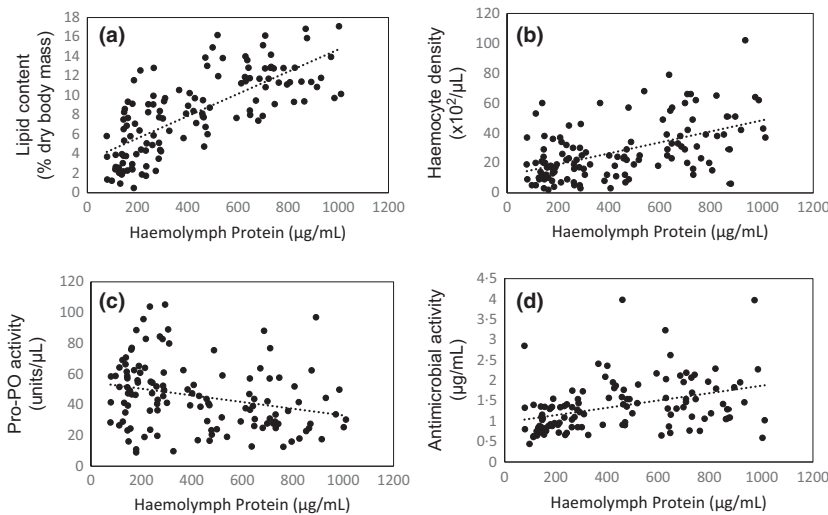
Figure 2 Interaction between haemolymph protein and immune traits in field-collected locusts. (a) Lipid content, (b) total haemocyte density, (c) prophenoloxidase activity and (d) lysozyme-like antimicrobial activity.
