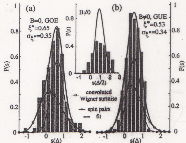
FIG. 2. Measured NNS distributions (gray bars) for B=0 (a) and B \neq 0 (b). The bold solid curves are the fits to P_{int}^\beta(\xi^*, \sigma_{\xi^*}) , with the fit results as indicated in the figure (see text). Also drawn are the two components of P_{int}^\beta , i.e. the Gaussian distribution of separations between spin pairs, and its convolution with the corresponding Wigner surmises. The inset compares the GUE data to P^2(s) (eq. 1), using the spin-resolved level spacing \Delta/2 as the average peak separation.
