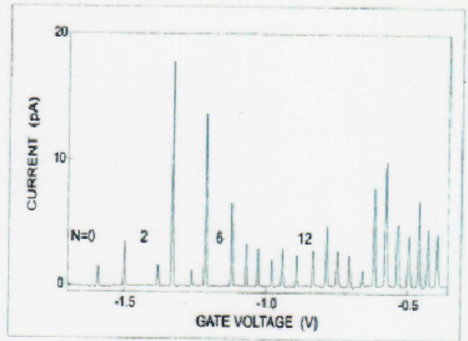
Coulomb oscillations
