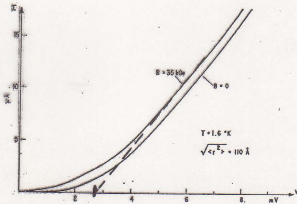
FIG. 7. Current-versus-voltage characteristic of a junction with average particle radius r=110 \text{ \AA} at 1.6^\circ\text{K} for H=0 (particles superconducting) and H=35 \text{ kOe} (particles normal).
