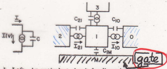
FIG. 1. Left: An equivalent circuit for discussion of charge effects for a single junction. Right: A comparable triple-junction circuit model.
