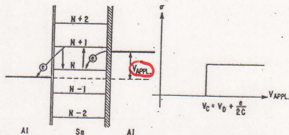
FIG. 13. Mechanism of current flow for an asymmetric junction ( C_L \gg C_B ). An electron from the right film tunnels into the particle, raising its electron number from N to N+1 and its voltage from V_D to V_D + e/C . In a next step the electron tunnels out onto the left film bringing the particle back in its ground state. This results in a step function for the conductivity as a function of voltage.
