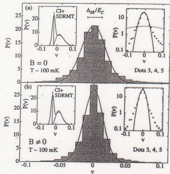
FIG. 2. Histograms of normalized peak spacing \nu (bars) for (a) B = 0 and (b) B \neq 0 for devices 3, 4, and 5. Solid curves show best fit to normalized Gaussian of width 0.019 (0.015) for B = 0 ( B \neq 0 ). The B = 0 histogram is wider by a factor of \sim 1.2 than the B \neq 0 histogram. Data represent 4300 (10 800) CB peaks from the devices with \sim 720 (1600) statistically independent for B = 0 ( B \neq 0 ). Horizontal bar indicates (spin-resolved) mean level spacing \Delta_{SR}/E_C averaged over the three devices. Right insets: Plots of histogram (diamonds) and best fit Gaussian (solid curve) on log-linear scale. Dashed curve is Gaussian of width 0.13 from Ref. [5]. Left insets: Dotted curves are CI + SDRMT peak spacing distributions; solid curves correspond to CI + SDRMT distributions convolved with Gaussian of width \sigma_{\text{noise}}(\nu) = 0.009 averaged over the three dots (see Table I).
