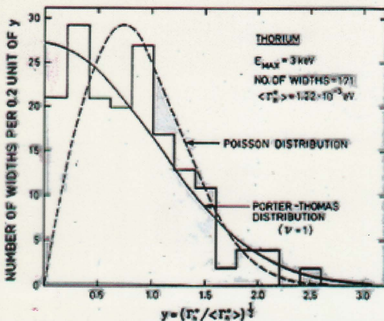
Figure 2-10 The figure plots the probability distribution of the reduced neutron widths observed in the reaction n + {}^{232}\text{Th} ( \Gamma_i^{(0)}(E) = \Gamma_i(E)E^{-1/2} (eV)). The data are taken from J. B. Garg, J. Rainwater, J. S. Petersen, and W. W. Havens, Jr., Phys. Rev. 134, B985 (1964).
