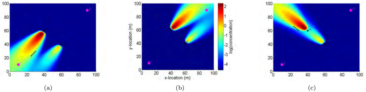
Fig. 1: Showing the log-concentrations for sensors at a height of 1 metre generated by a Gaussian plume for a particular wind field. The black dots show the locations of two circular methane sources of radius 1m; the source labelled A is emitting at a rate of 100 kg/hr, and the one labelled B at a rate of 20 kg/hr. The magenta dots labelled C and D correspond to possible sensor locations.
