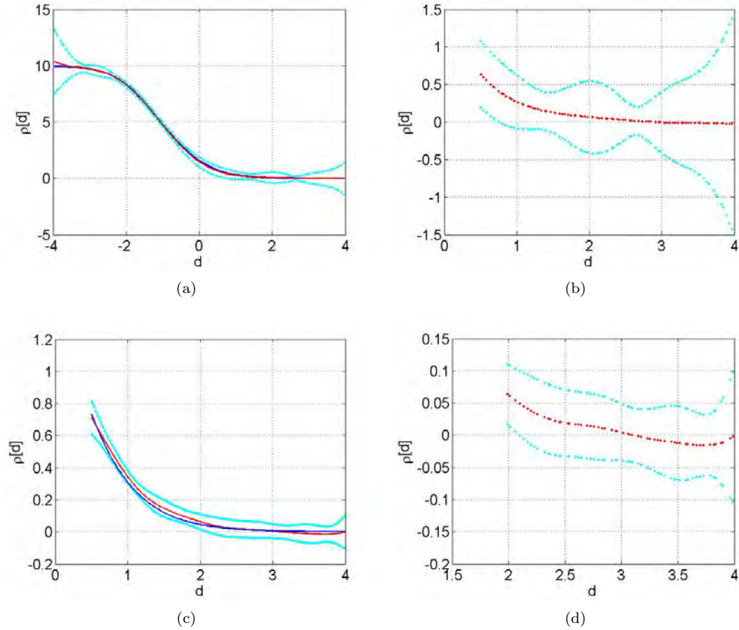
Fig. 3: Plots of the design space reduction process for the linear model example discussed in 5; red (mean) and cyan (2 std. dev. error bars) indicate predictions from the Bayes linear emulator, whereas blue indicates results obtained by ‘brute force’ numerical integration of the risk (7) over w . 3(a) shows the emulator at wave 1, fitted to samples drawn from risks such as those in 2 and integrated over w ; 3(b) shows a set of d values sampled from the non-implausible space defined by this emulator; figure 3(c) then shows the wave 2 emulator fitted to this non-implausible space using data sampled at the design points in 3(b); figure 3(d) shows the risk at a set of values of d sampled from the non-implausible space defined by both the wave 1 and wave 2 emulators (3(a) and 3(c)). Note that the size of the remaining design space and the upper bound for the minimum risk both decrease as we perform each wave.
